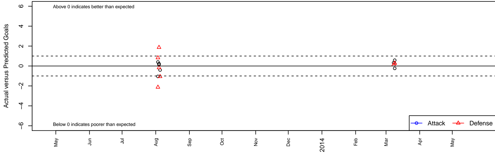
Real Colorado National G01 Dots are actual minus expected GF (blue circles) and GA (red triangles). Blue line is smoothed change in attack strength. Red is smoothed change in defense strength.
